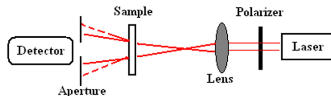
Fig. 2. Experimental set-up for the closed aperture Z-scan technique.
